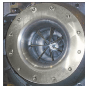
Figure 4 – Inlet Guide Vane Mechanical Losses Increase as the Vanes Close
